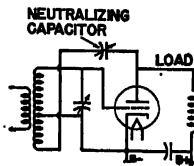
Neutralizing capacitor used to cancel feedback.
